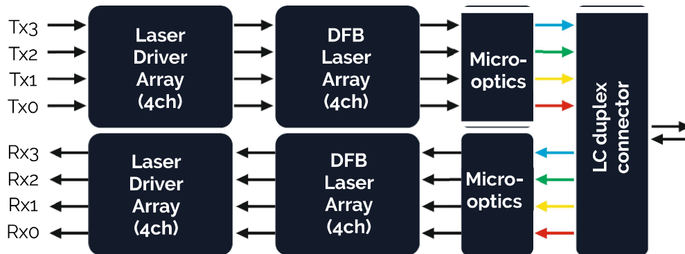
Figure 1. Functional diagram
