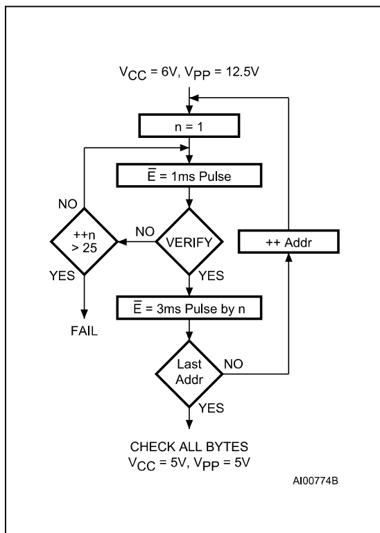
Figure 7. Programming Flowchart
