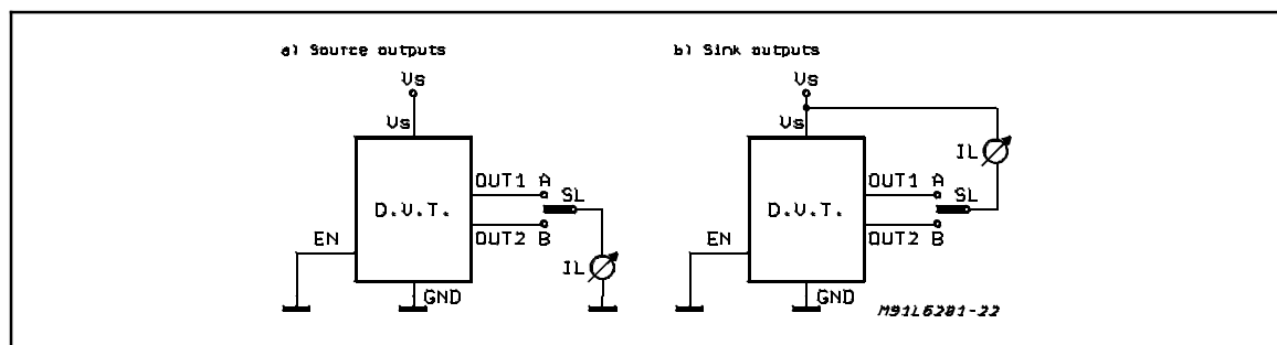
Figure 11: Leakage Current
