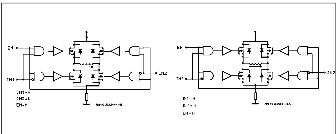
Figure 8c: Enable Chopping
