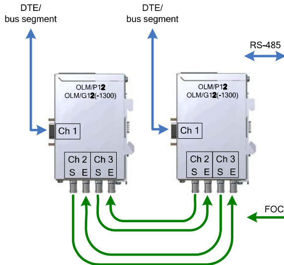
Figure 3-2 Configuration 1
