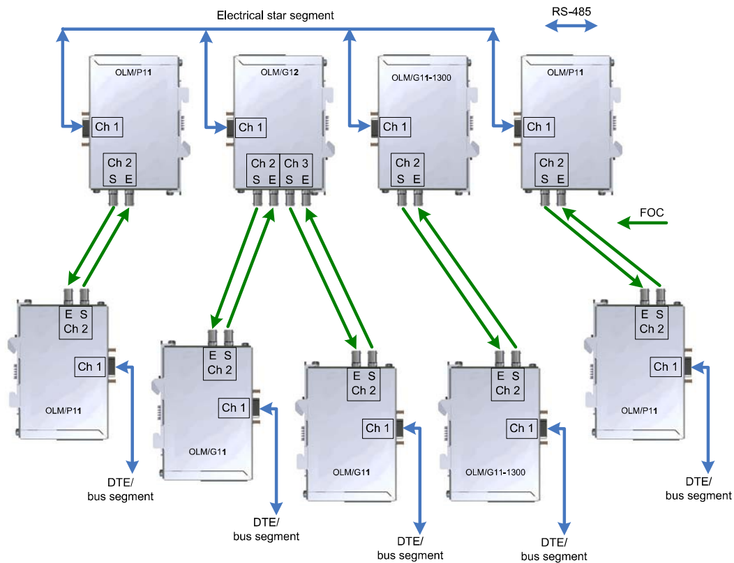
Figure 3-2 Network structure with an optical star topology
