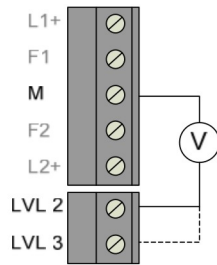
Figure 5-11 Position of the level recording connections
