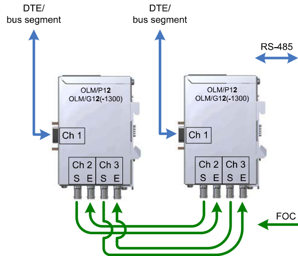
Figure 3-1 Configuration 2
