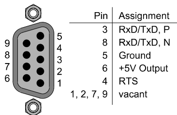
Figure 5-7 Electrical port, connector assignment D-sub jack
