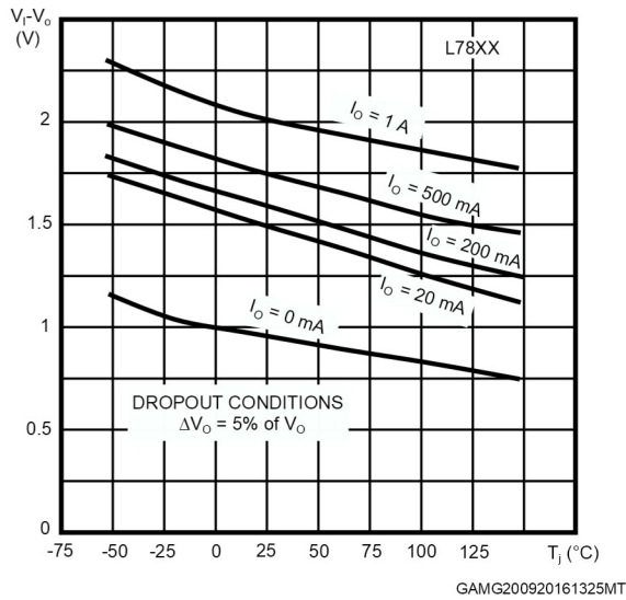
Figure 28. Dropout voltage vs junction temperature
