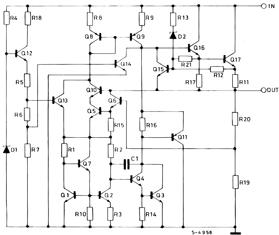
Figure 3. Schematic diagram
