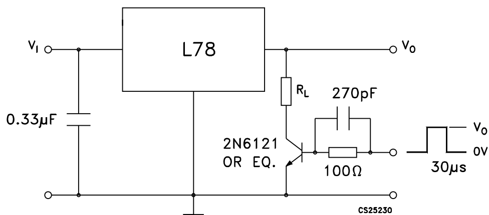
Figure 6. Load regulation
