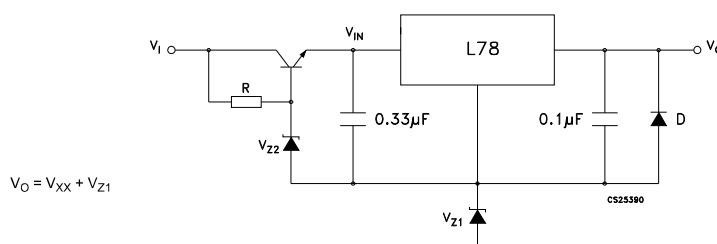
Figure 21. High input and output voltage
