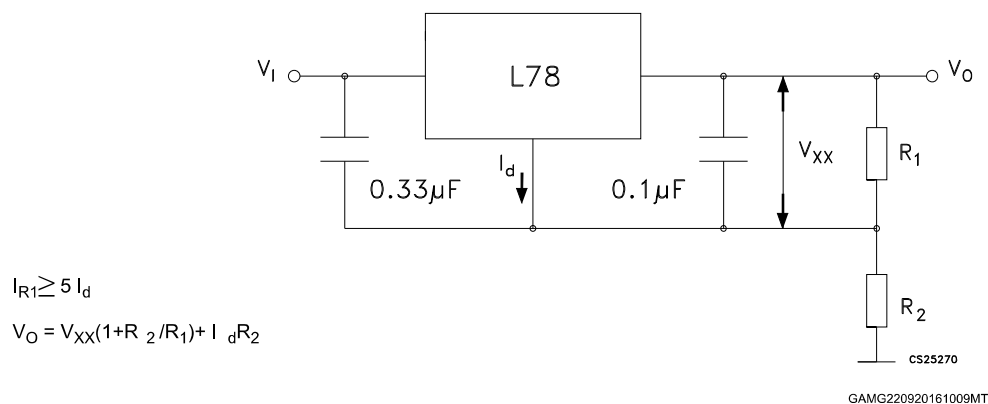
Figure 11. Adjustable output regulator (7 to 30 V)
