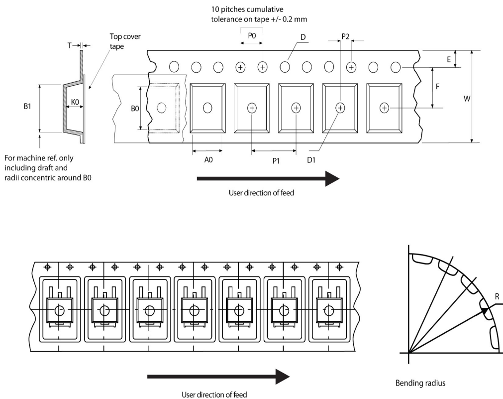
Figure 47. Tape outline
