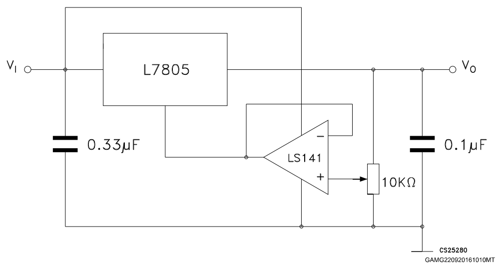
Figure 11. Adjustable output regulator (7 to 30 V)
