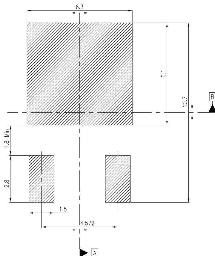
Figure 43. DPAK recommended footprint (dimensions are in mm)
