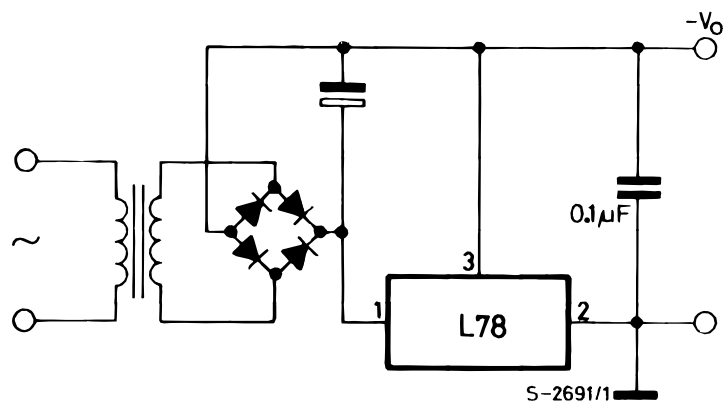
Figure 17. Negative output voltage circuit
