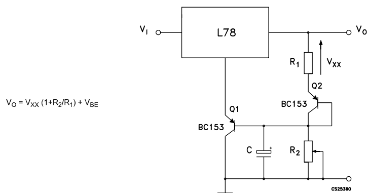
Figure 25. Adjustable output voltage with temperature compensation
