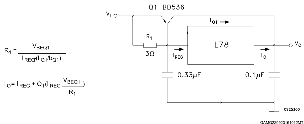
Figure 14. High output current with short circuit protection
