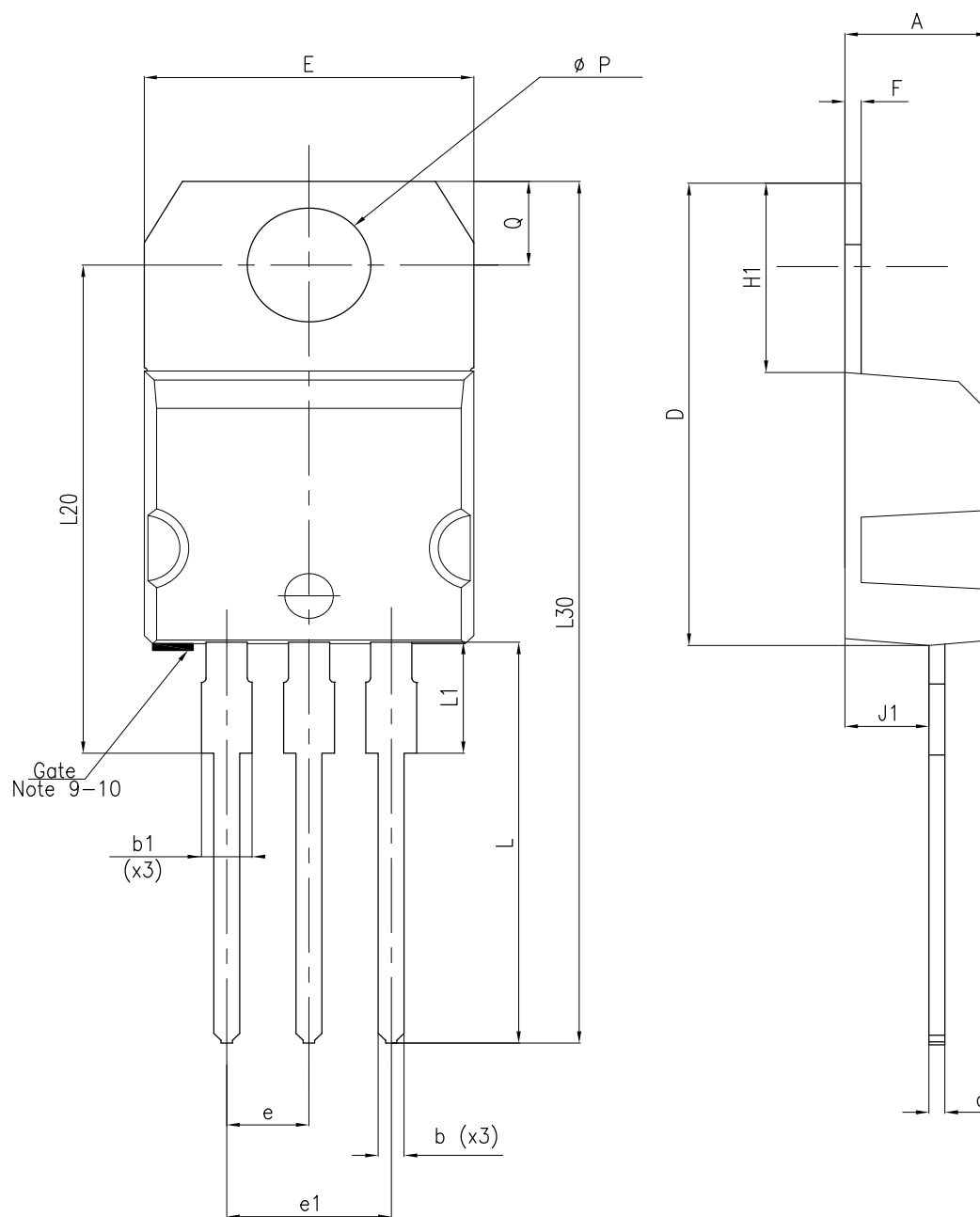
Figure 38. TO-220 (single gauge) package outline
