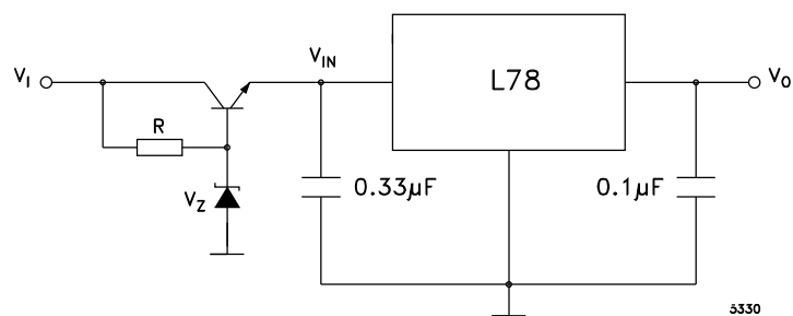
Figure 21. High input and output voltage
