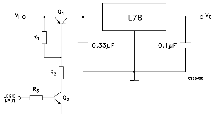
Figure 23. Remote shutdown
