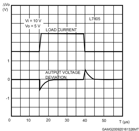
Figure 34. Load transient response
