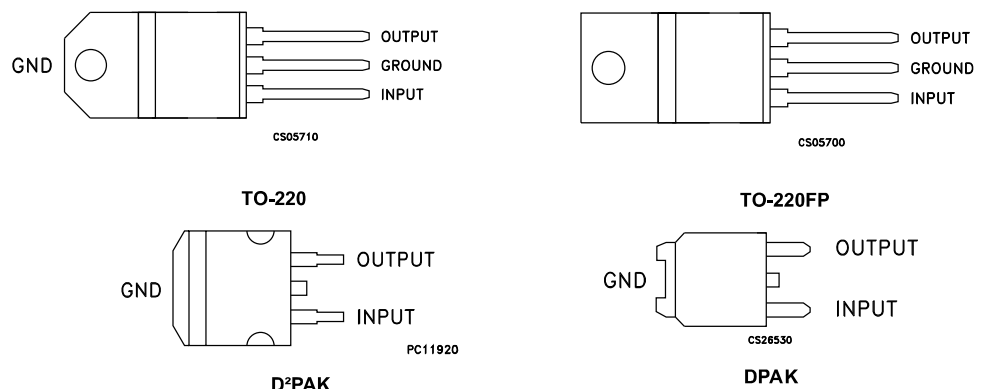
Figure 2. Pin connections (top view)
