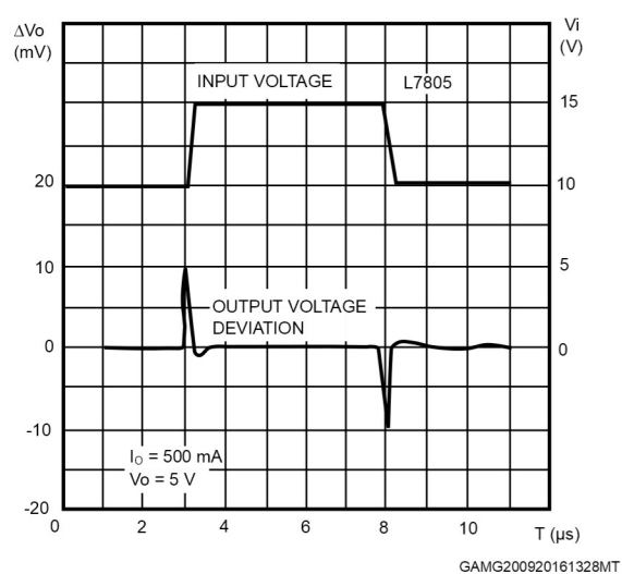
Figure 35. Line transient response
