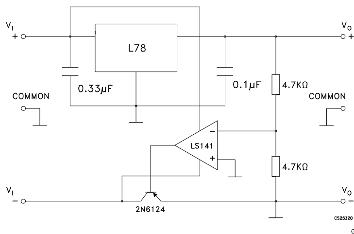
Figure 16. Split power supply ( \pm 15\text{ V} - 1\text{ A} )
