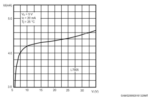
Figure 36. Quiescent current vs. input voltage
