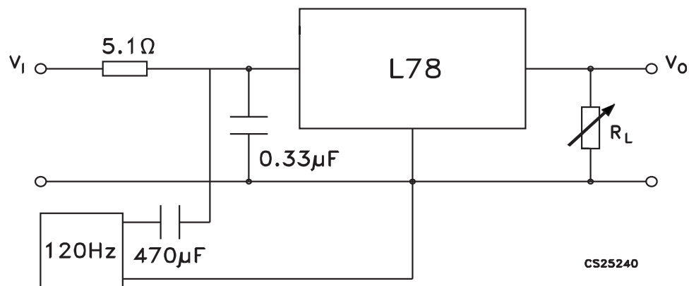
Figure 7. Ripple rejection
