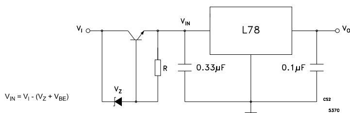
Figure 19. High input voltage circuit (configuration 1)
