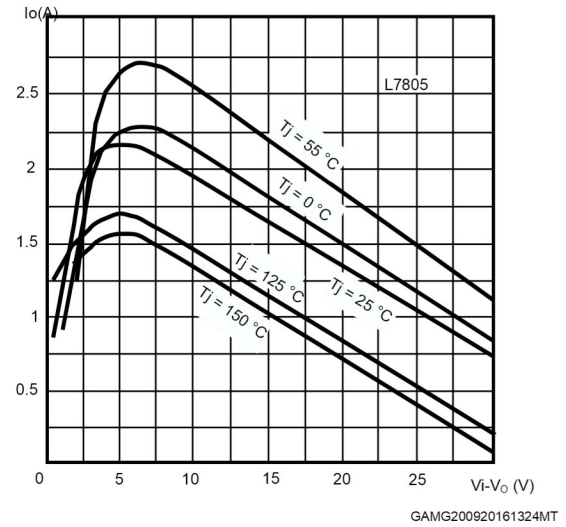
Figure 29. Peak output current vs input/output differential voltage
