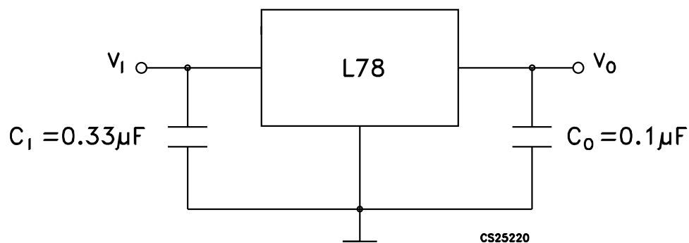
Figure 4. Application circuits
