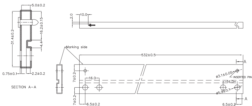
Figure 41. Tube for TO-220 (single gauge) (mm.)
