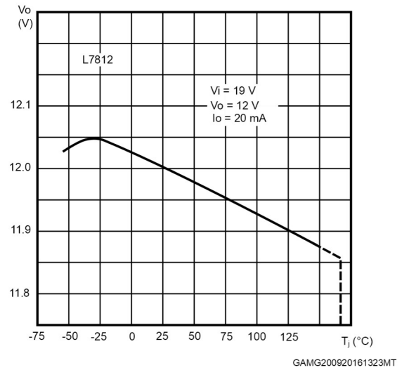
Figure 31. Output voltage vs junction temperature
