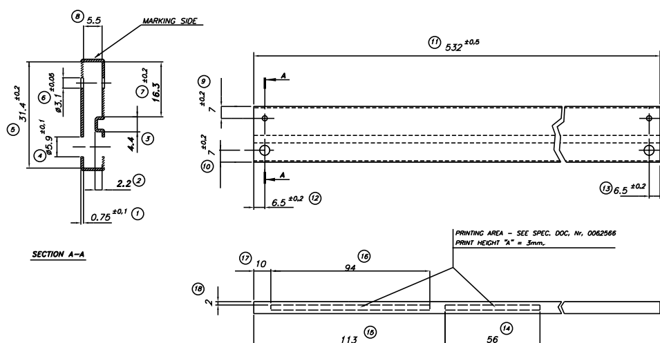
Figure 40. Tube for TO-220 (dual gauge) (mm.)
