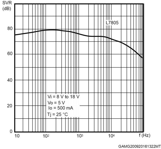
Figure 30. Supply voltage rejection vs frequency
