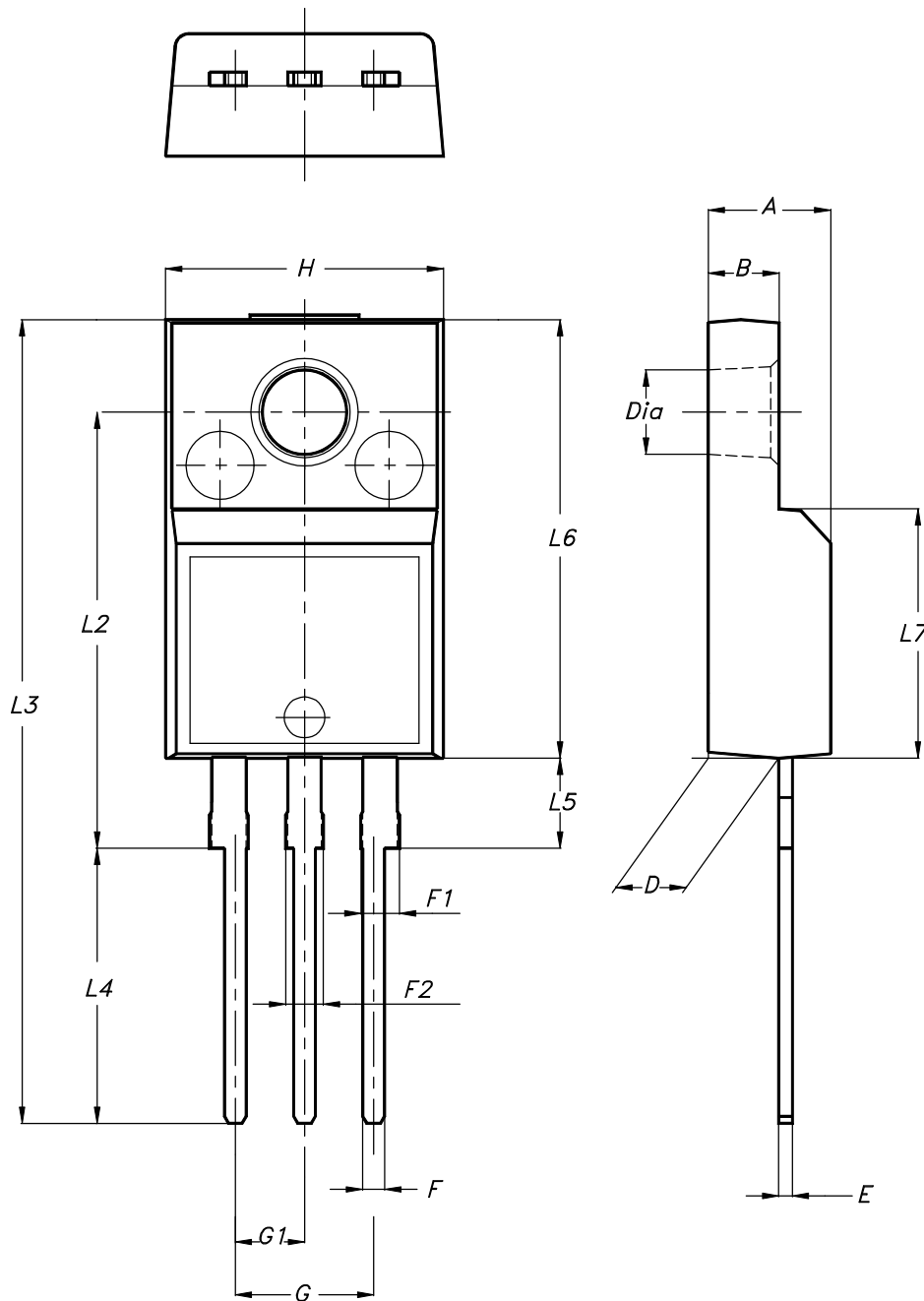
Figure 39. TO-220FP package outline
