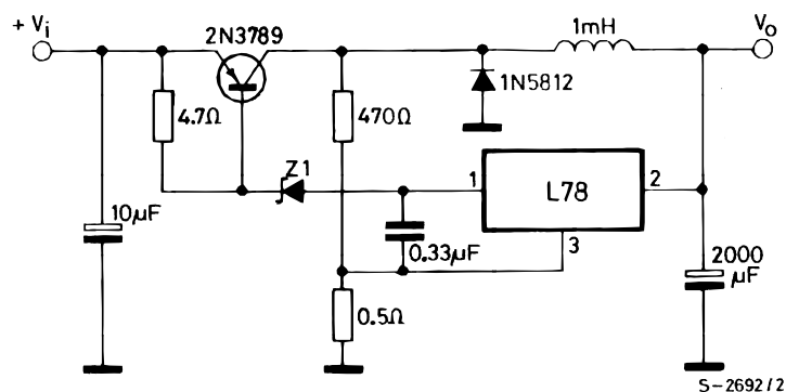
Figure 19. High input voltage circuit (configuration 1)
