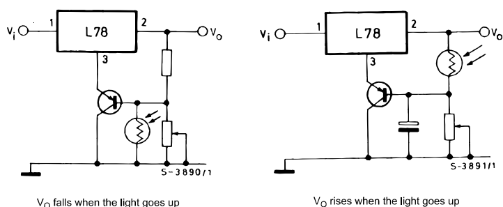
Figure 26. Light controllers ( V_{O(min)} = V_{XX} + V_{BE} )
