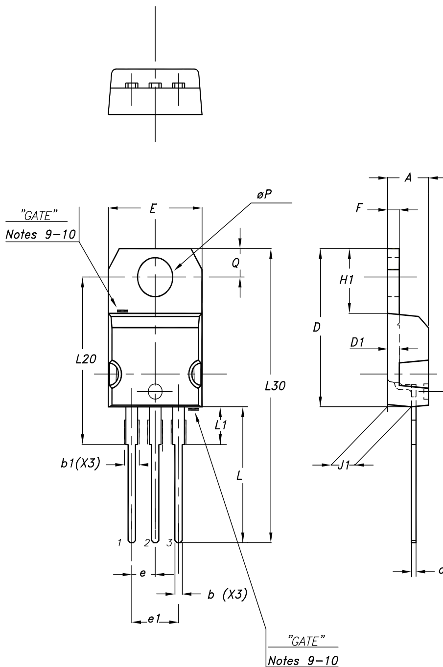
Figure 37. TO-220 (dual gauge) package outline
