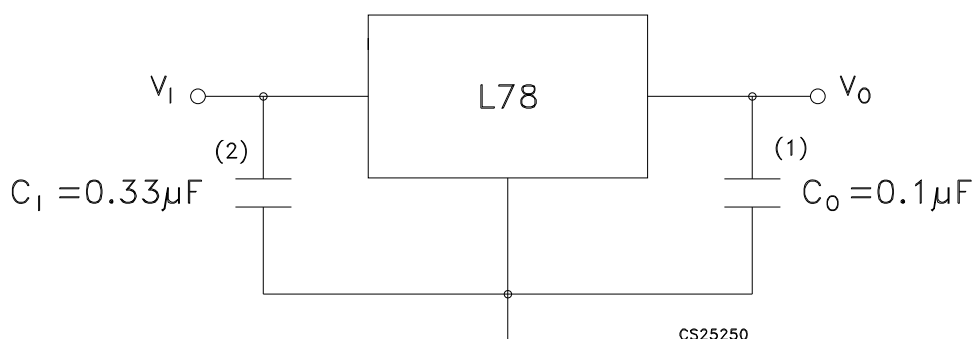
Figure 8. Fixed output regulator
