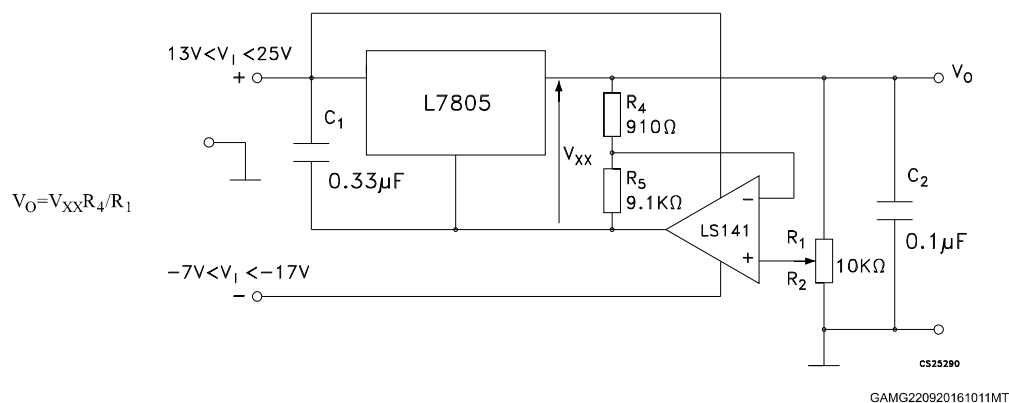
Figure 13. High current voltage regulator
