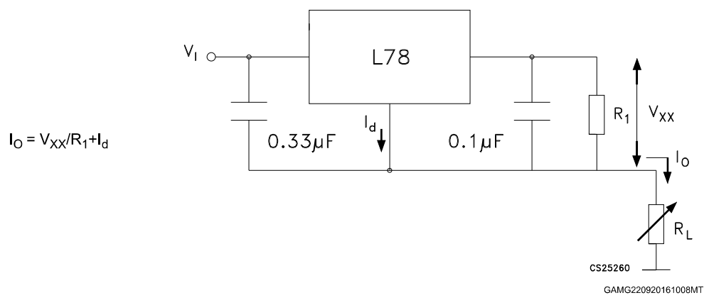
Figure 10. Circuit for increasing output voltage
