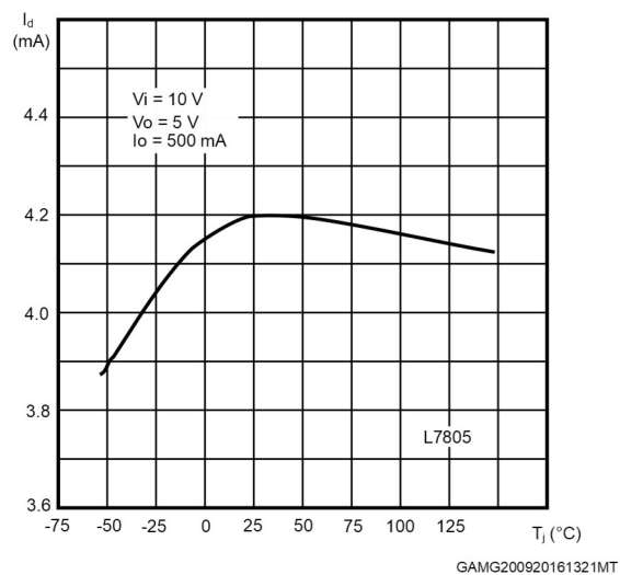
Figure 33. Quiescent current vs junction temp.
