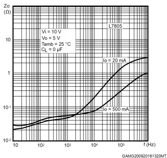
Figure 32. Output impedance vs frequency
