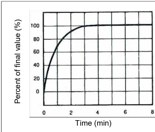
Figure 10. Thermal response in still air
