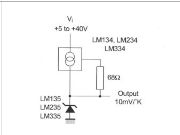
Figure 14. Wide operating supply
