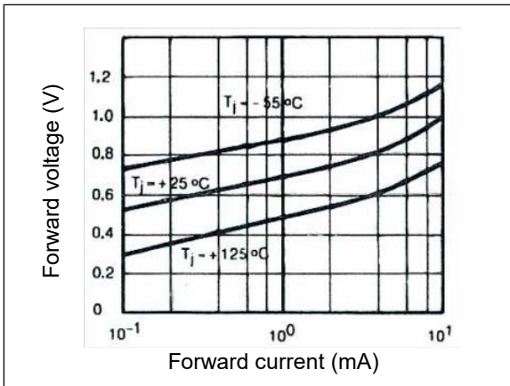
Figure 12. Forward characteristics
