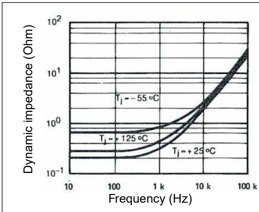
Figure 6. Dynamic impedance
