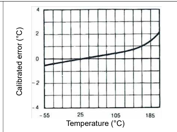
Figure 3. Calibrated error
