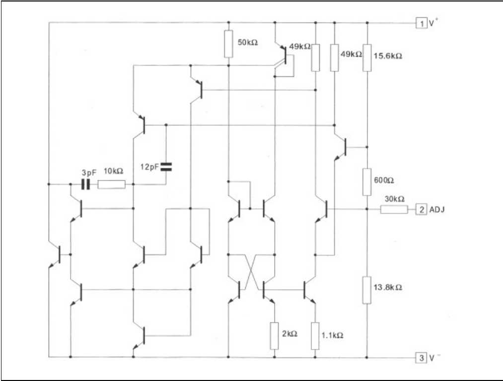
Figure 1. Schematic diagram
