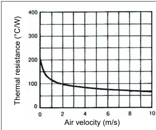
Figure 8. Thermal resistance junction to air
